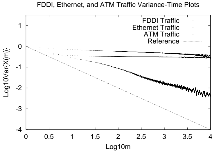
Figure 5: LRD Traffic in Three Different Network Types.
