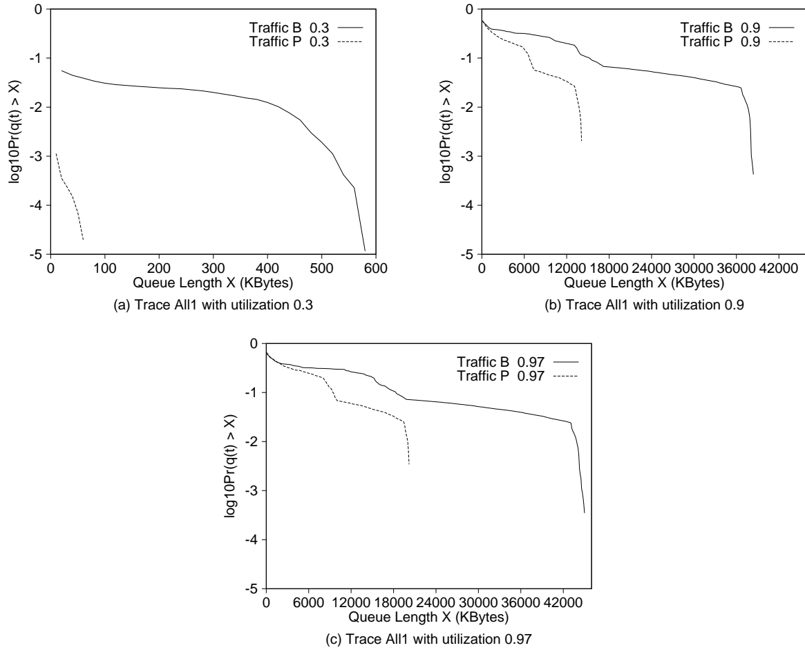
Figure 12: Queueing experiments for trace All1 with 0.3, 0.9 and 0.97 utilizations.
