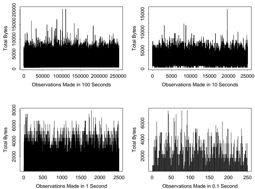
Figure 2: CSD Traffic Trace Over Many Time Scales.
