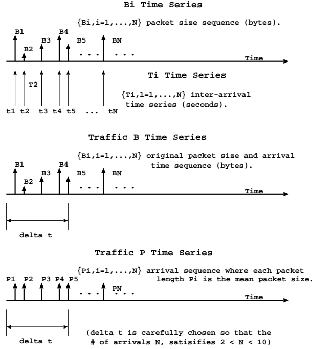
Figure 3: Time Series Diagrams.
