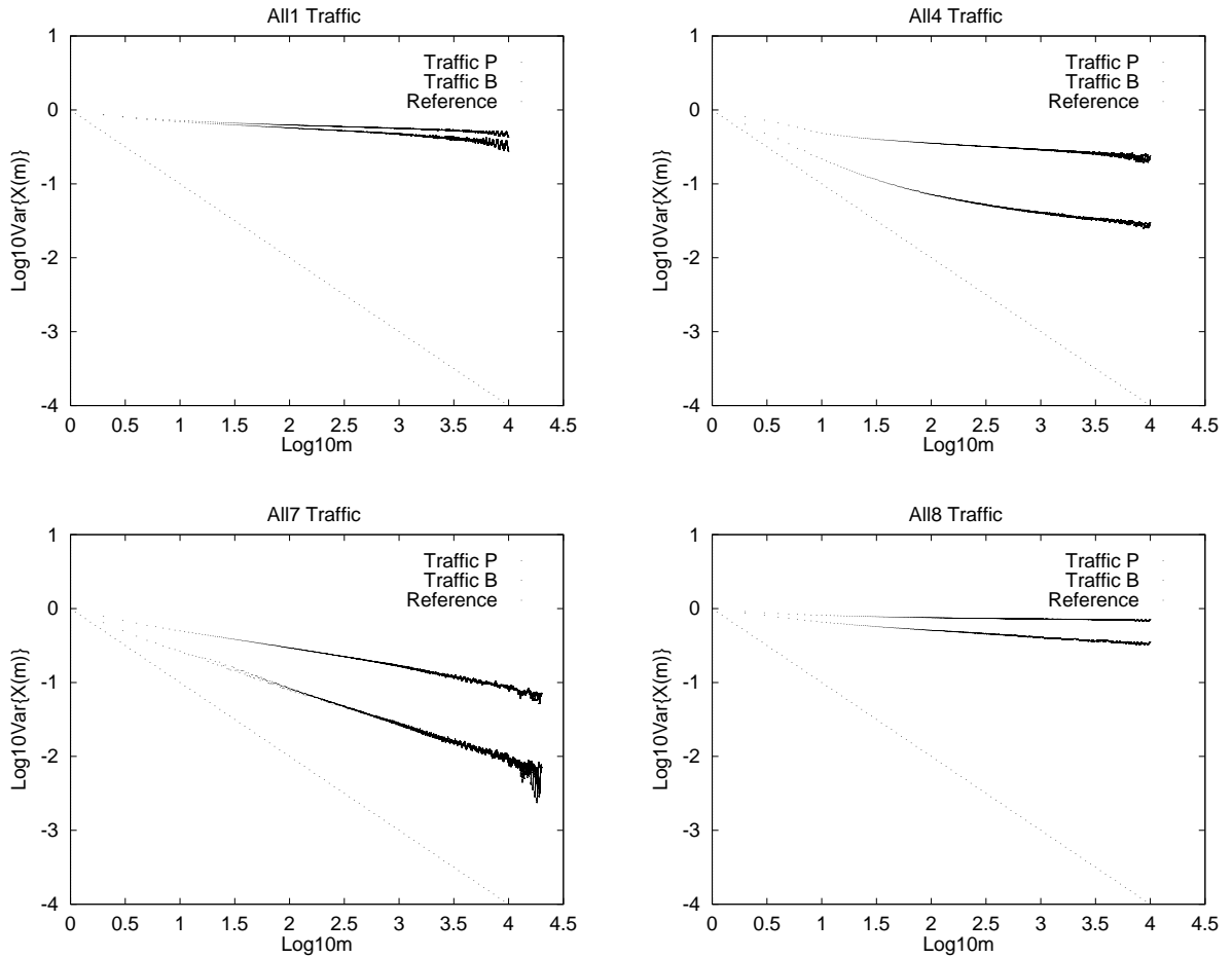
Figure 6: Variance-time plots for the 4 traces.
