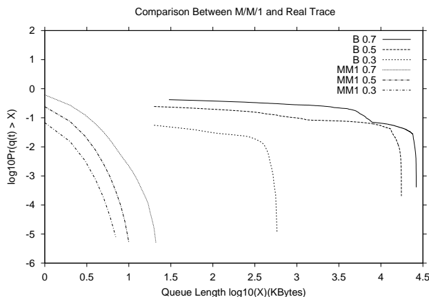
Figure 8: Queueing experiment for M/M/1 model and the LRD All1 trace.
