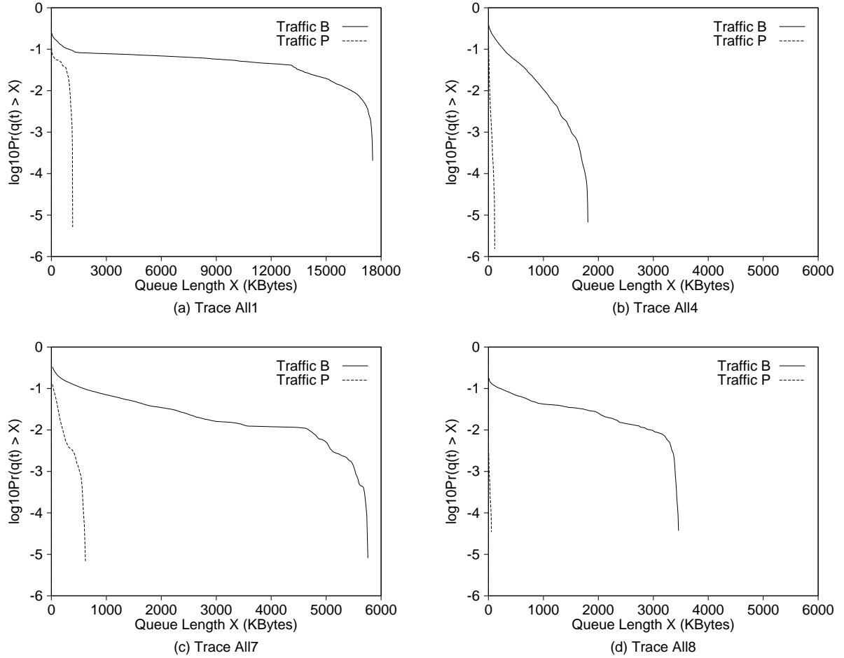
Figure 11: Queueing experiment of each trace with 0.5 utilization.
