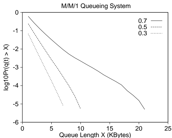
Figure 7: Queueing experiment for M/M/1 model using \lambda and \mu from All1 trace.
