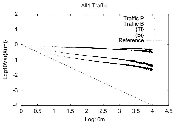
Figure 4: Variance-time plots for all 4 timeseries.
