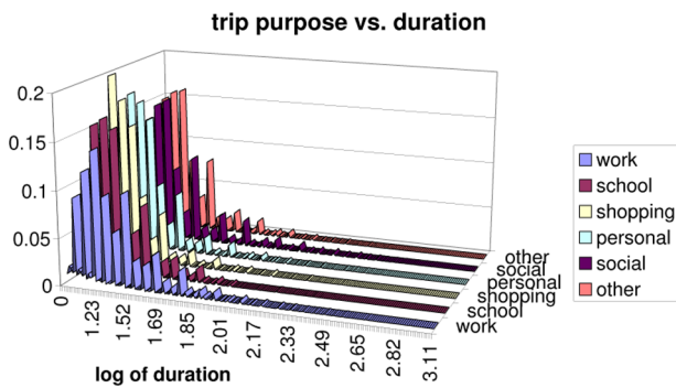
Figure 3 Trip duration distribution (see online version for colours)
