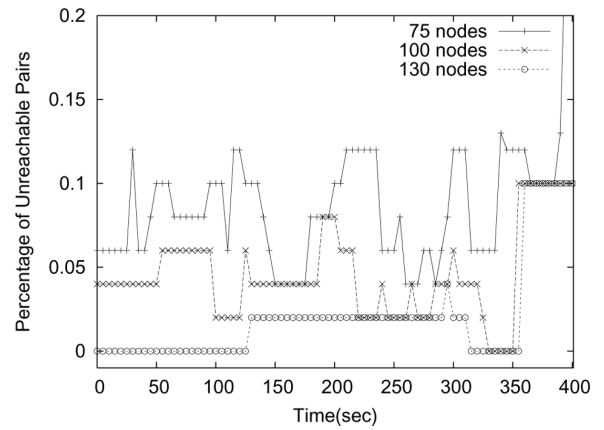
Figure 19 Unreachable pairs in 15 min, from 8:45 AM to 9:00 AM
