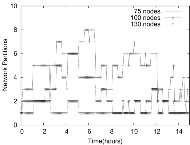
Figure 18 Number of partitions in 15 h
