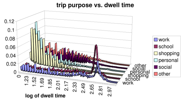
Figure 5 Dwell distribution (see online version for colours)
