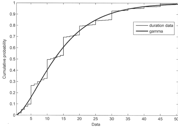
Figure 7 Fit Gamma distribution to trip duration data
