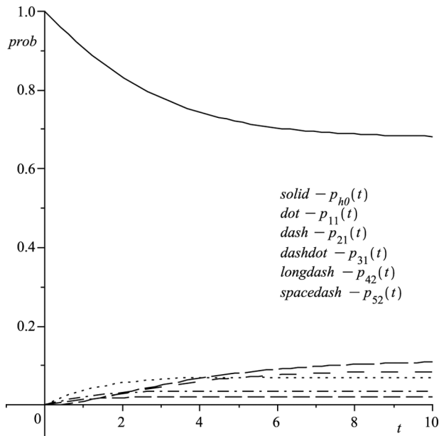
Figure 12 Numerical solution: state probabilities
