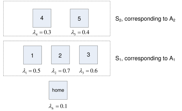
Figure 10 A node starting from home has an agenda consisting of activities A_1 and A_2 . There are five locations (plus home). To conduct activity A_1 , the node select one (and only one) location from location set S_1 = \{1, 2, 3\} ; to conduct activity A_2 , it selects one from set S_2 = \{4, 5\} . The node staying at location i for exponential time with parameter \lambda_i . It returns home after it finishes activity A_2 . This procedure loops (see online version for colours)
