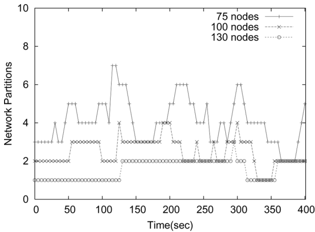
Figure 17 Number of partitions in 15 min, from 8:45 AM to 9:00 AM
