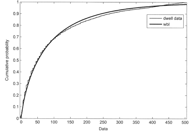
Figure 8 Fit Weibull distribution to dwell time data
