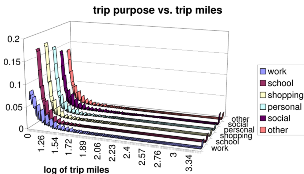
Figure 4 Mileage distribution (see online version for colours)
