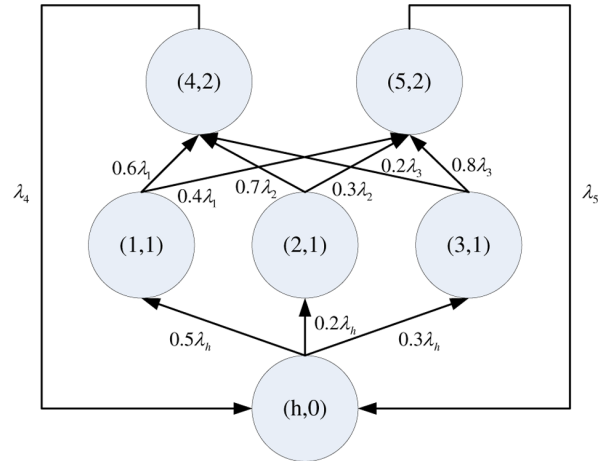
Figure 11 Continuous time markov chain state transition (see online version for colours)
