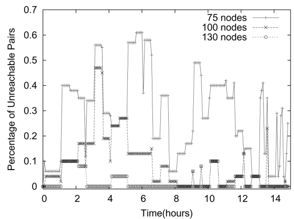
Figure 20 Unreachable pairs in 15 h
